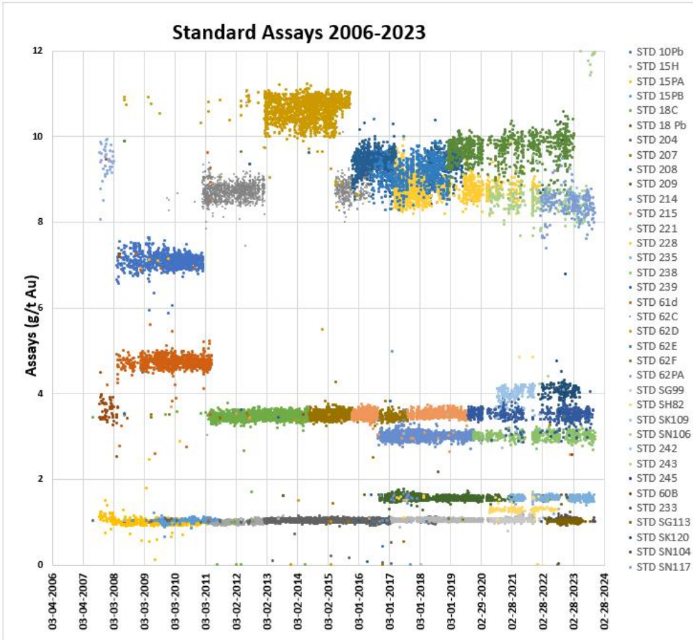
Figure STYLEREF 1 \s 8-. Plots of All CRM Assay Results from 2006 to 2023
