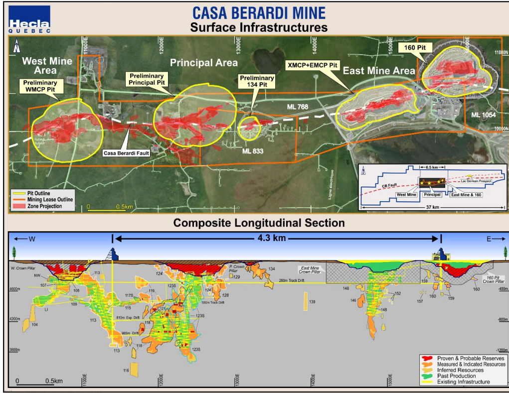
Figure STYLEREF 1 \s 11-. Mine Plan View and Composite Longitudinal Section of Deposit Areas and Infrastructure (from Hecla, 2023)
