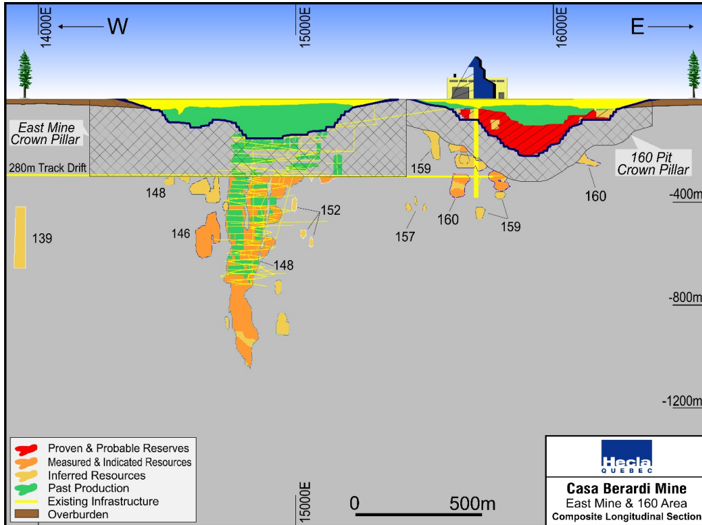
Figure STYLEREF 1 \s 6-. East Mine Composite Longitudinal Section
