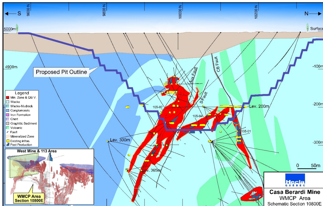
Figure STYLEREF 1 \s 6-. Section 10,800E, West Mine Geology and Mining Infrastructure
