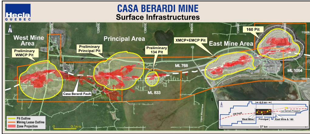
Figure STYLEREF 1 \s 3-. Plan View of Current and Planned Infrastructure (from Hecla, 2023)
