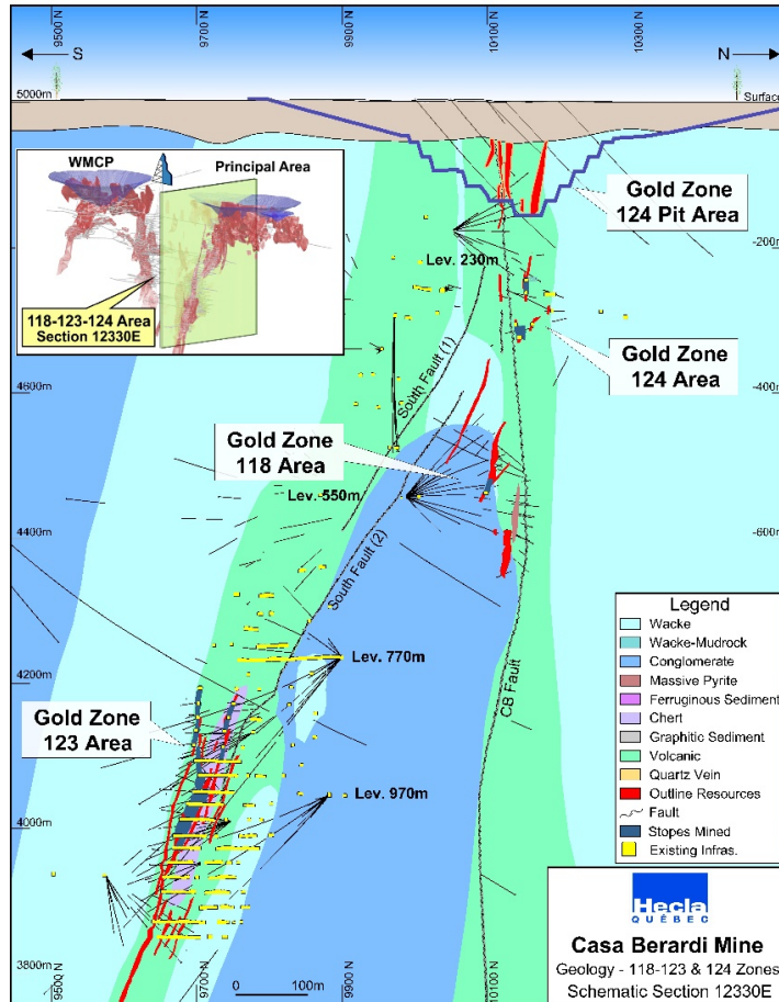
Figure STYLEREF 1 \s 6-. Section 12,330E, Principal Area Geology 118, 123, and 124 Zones
