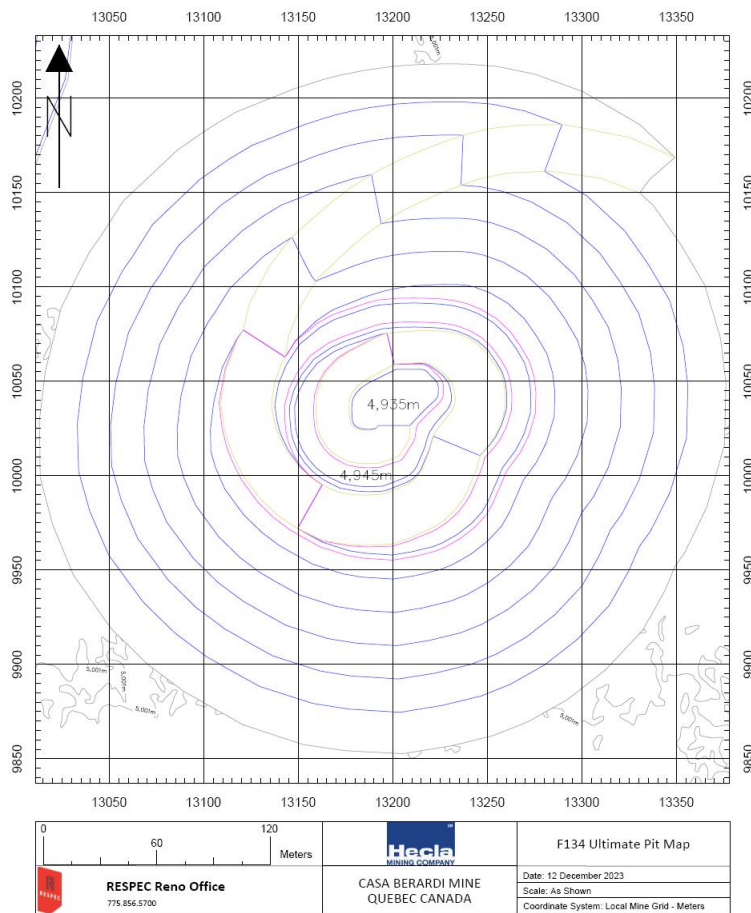
Figure STYLEREF 1 \s 13-. Plan View of the F134 Pit (Ultimate Pit Shell)
