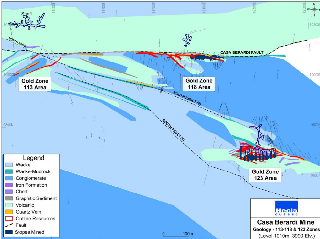
Figure STYLEREF 1 \s 6-. Plan View of the 1,010m Level, Principal Area
