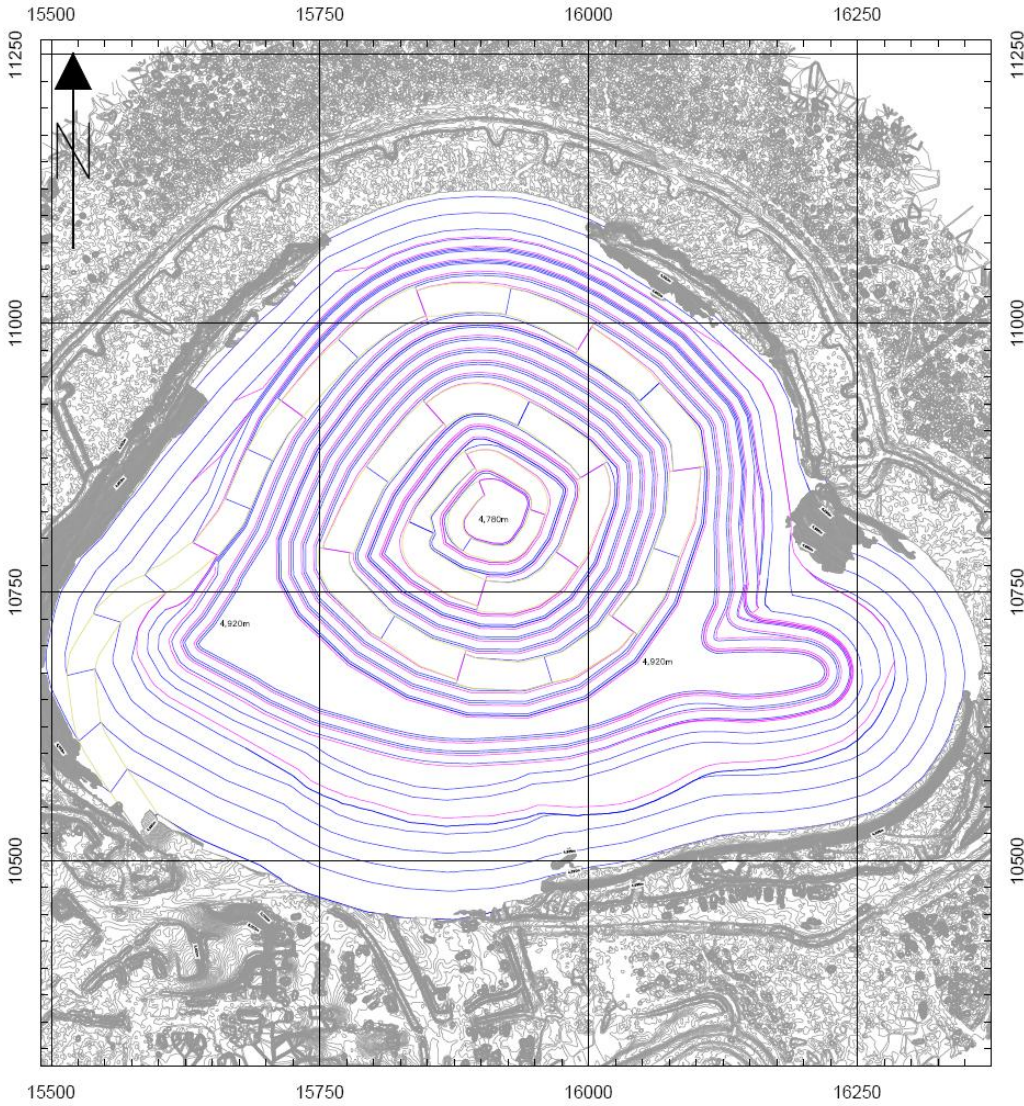
Figure STYLEREF 1 \s 13-. Plan View of the F160 Pit Project
