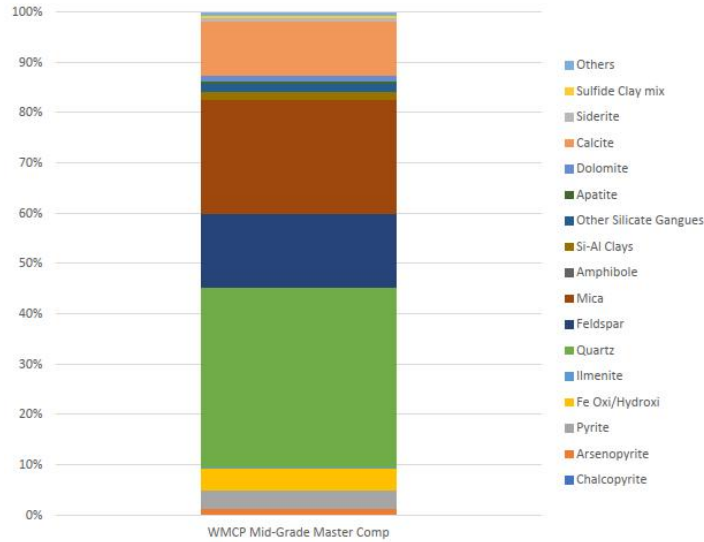
Figure STYLEREF 1 \s 10-. Mineralogical Analyses on Composites
