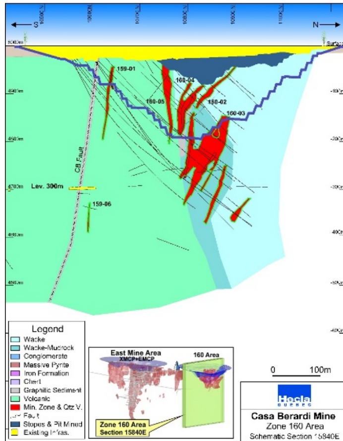
Figure STYLEREF 1 \s 6-. Section 15, 840E, East Mine Geology and Infrastructure – 160 Zone
