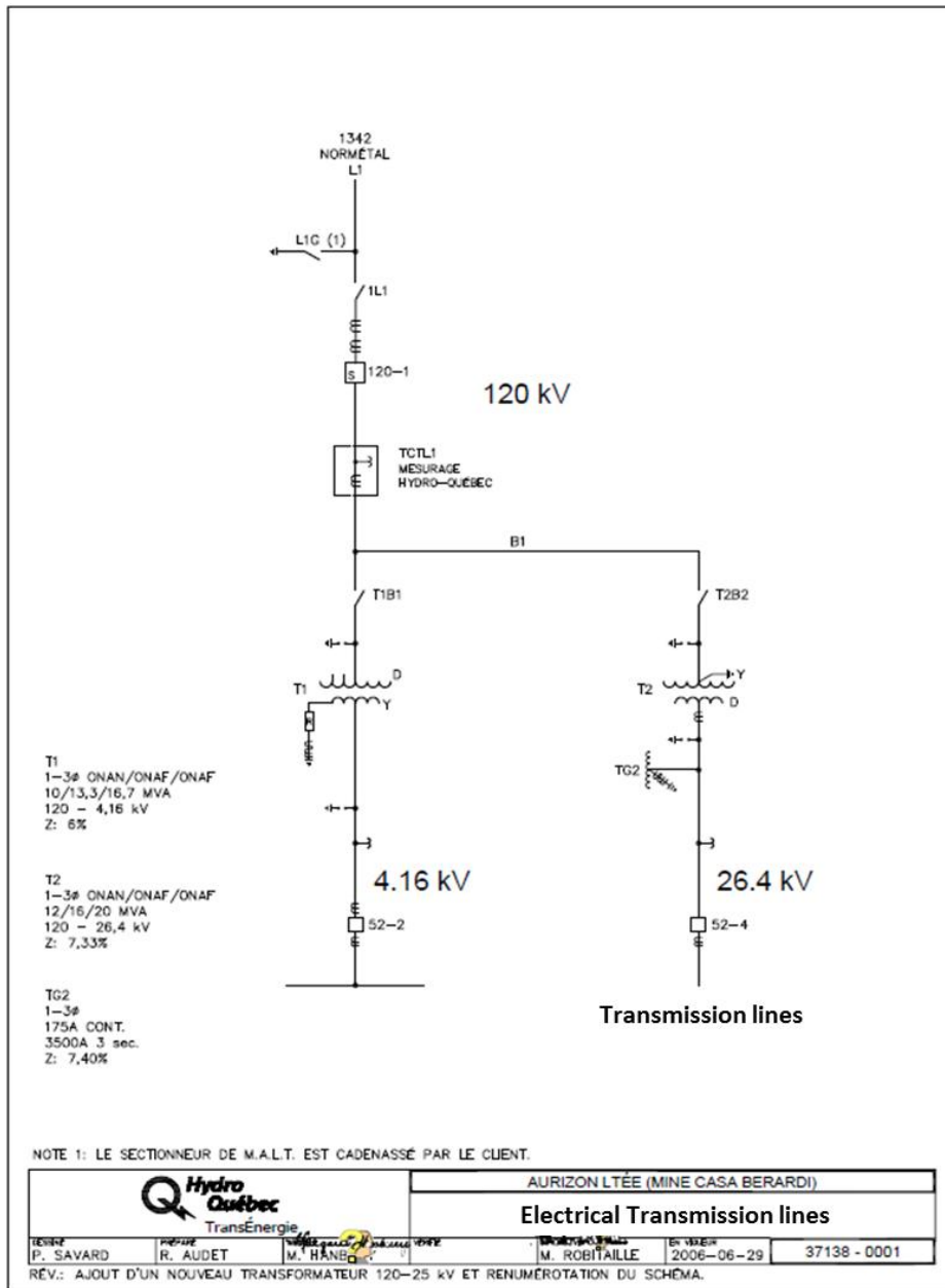
Figure STYLEREF 1 \s 13-. Casa Berardi Main Station 120kV Flowsheet
