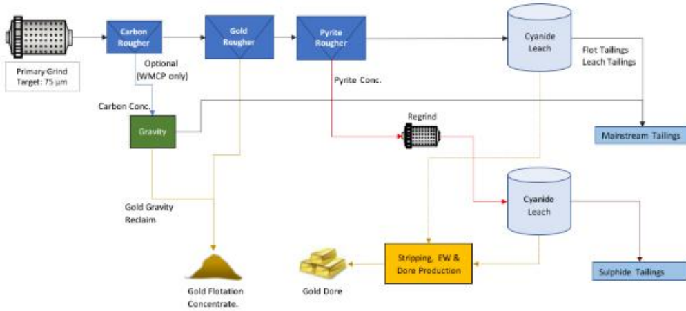
Figure STYLEREF 1 vs 10-. WMCP Blend Simplified Integrated Flowsheet
