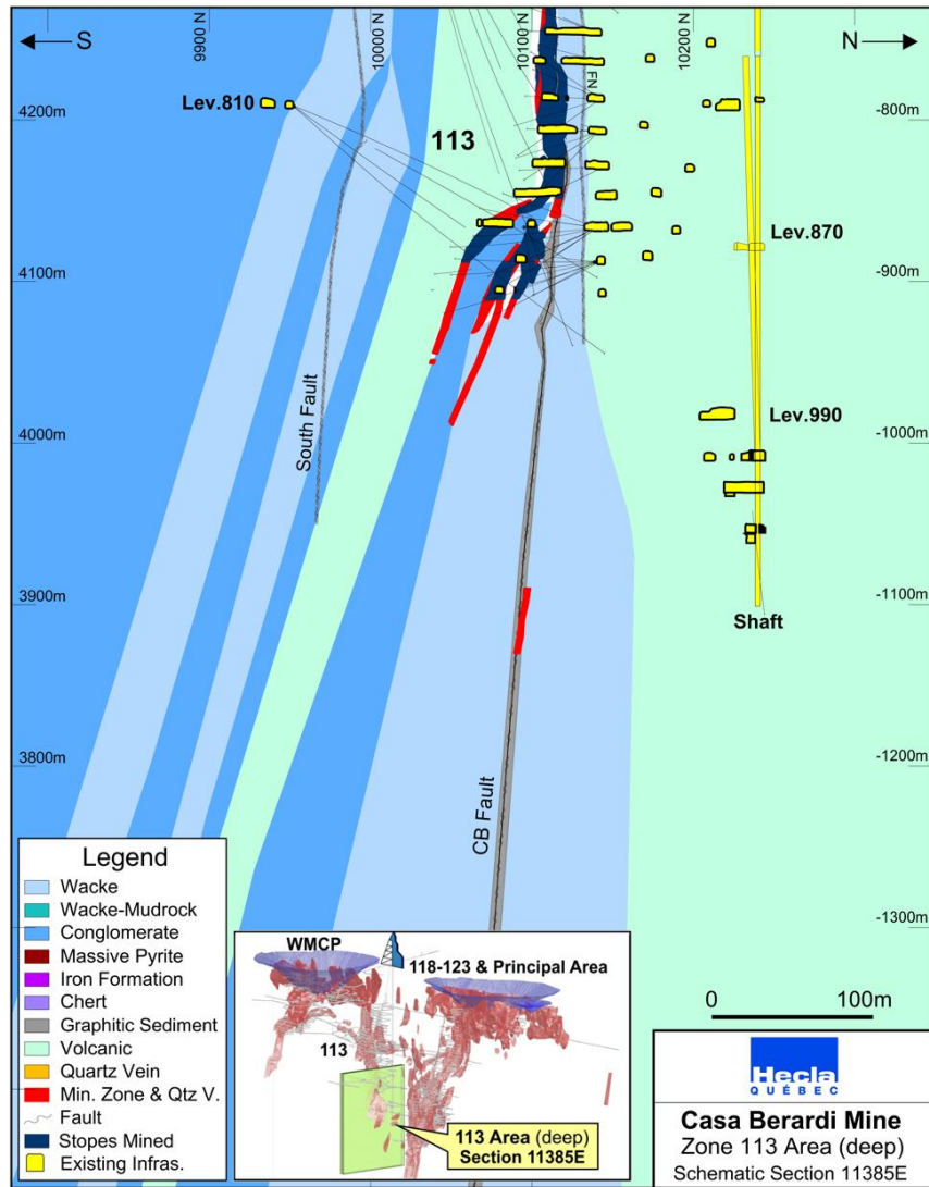
Figure STYLEREF 1 \s 6-. Section 11,385E, West Mine Including the 113 Zone and Casa Berardi Fault (from Hecla, 2023; Note that metamorphosed rocks are referred to by protolith nomenclature)
