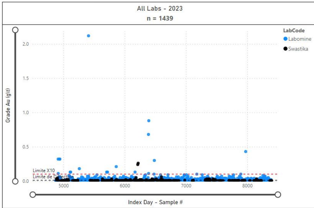
Figure 8-7. Mine and Swastika Blanks – 2023
