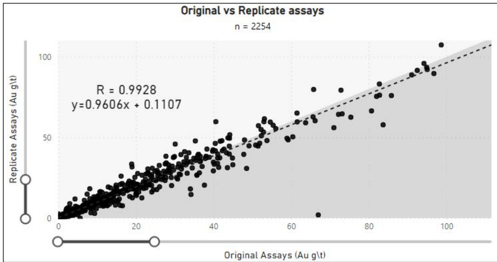
Figure STYLEREF 1 \s 8-. Mine Laboratory Pulp Duplicate Assays from 2021- 2023 (Assays below 120g/t Au)
