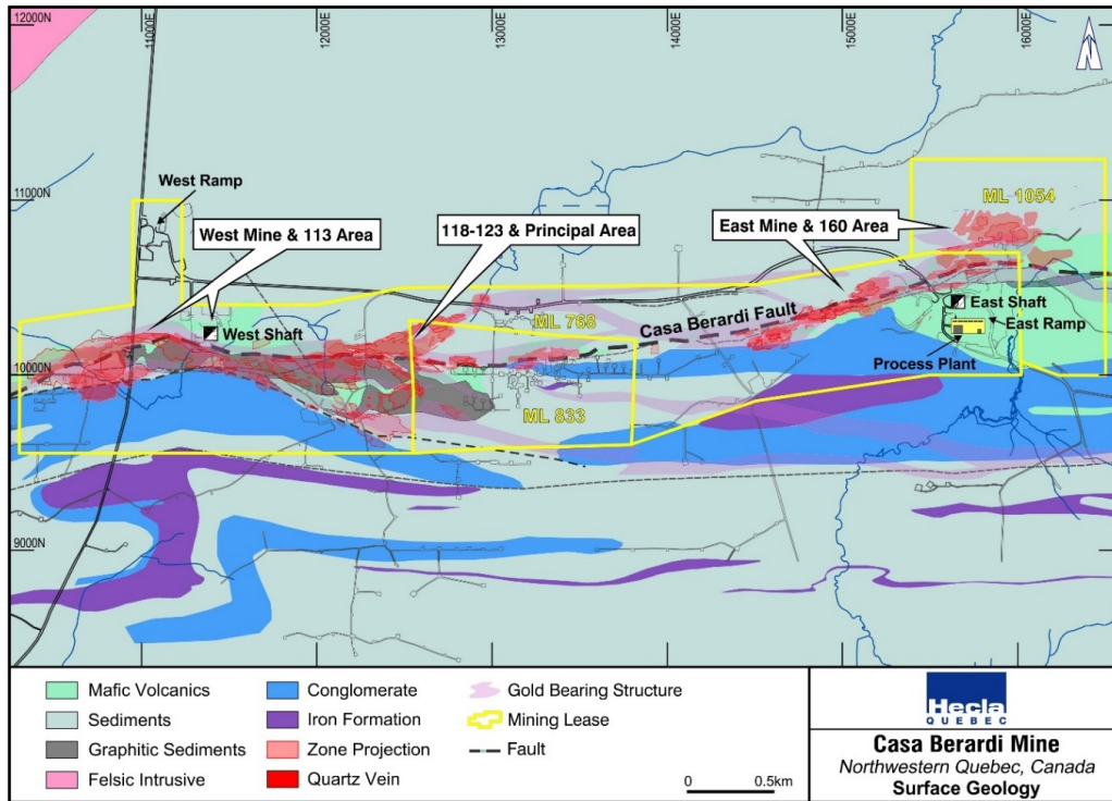
Figure STYLEREF 1 \s 6-. Mine Area Surface Geology
