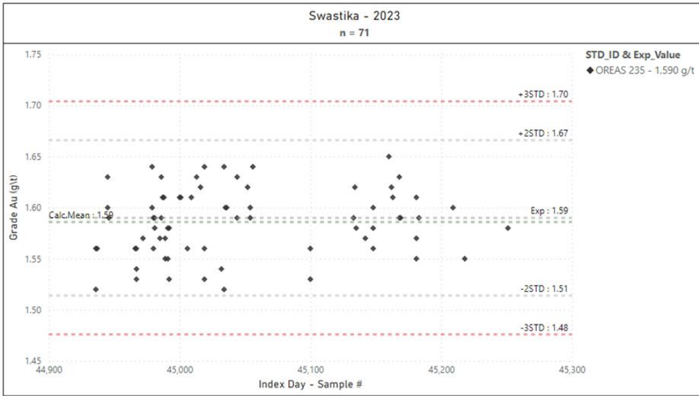
Figure STYLEREF 1 \s 8-. Plot of 2023 CRM Assays from Swastika for OREAS 235
