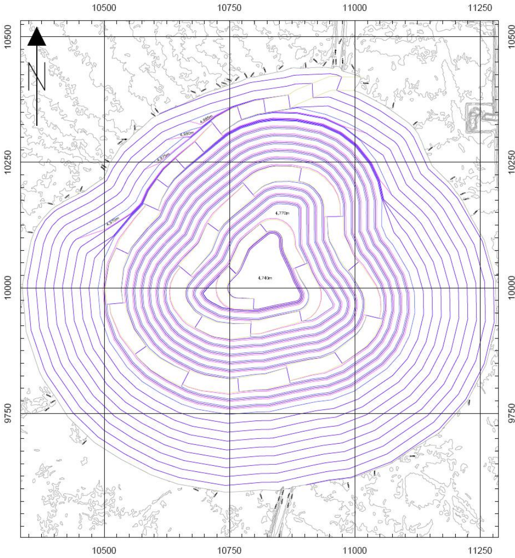
Figure STYLEREF 1 \s 13-. Plan View of the WMCP Pit Project (Ultimate Pit Shell)
