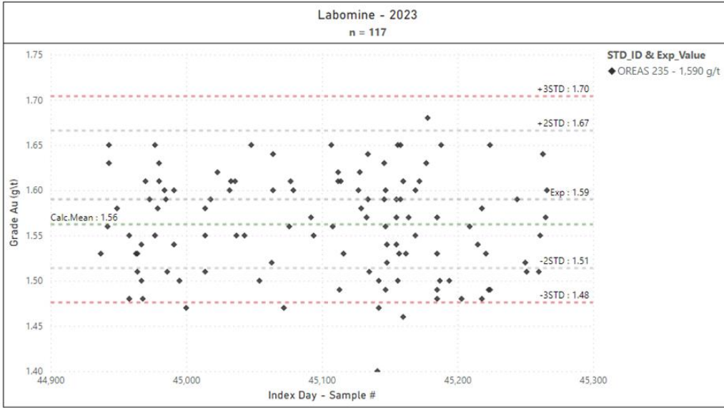
Figure STYLEREF 1 vs 8-. Plot of 2023 CRM Assays from the Mine Lab for OREAS 235
