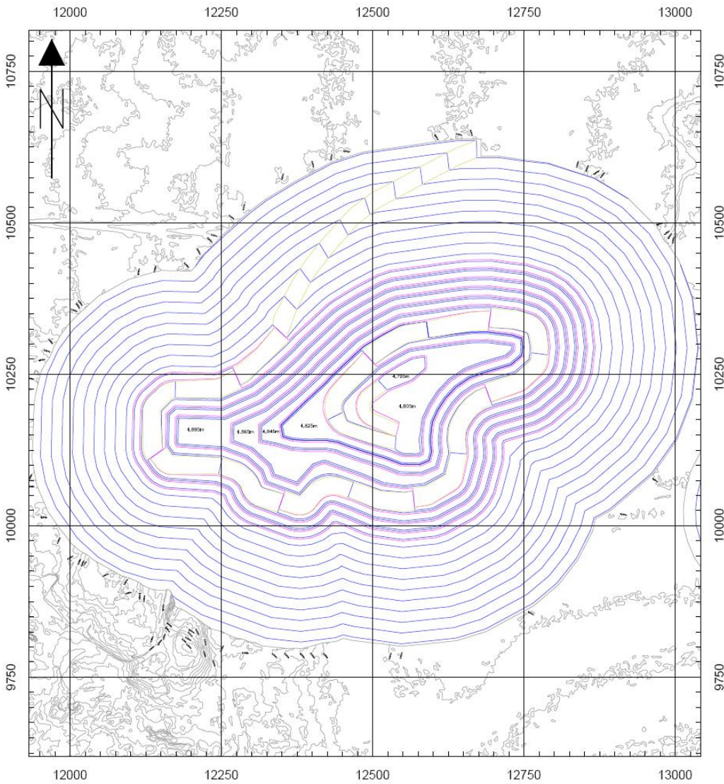
Figure STYLEREF 1 \s 13-. Plan View of the Principal Pit Project (Ultimate Pit Shell)
