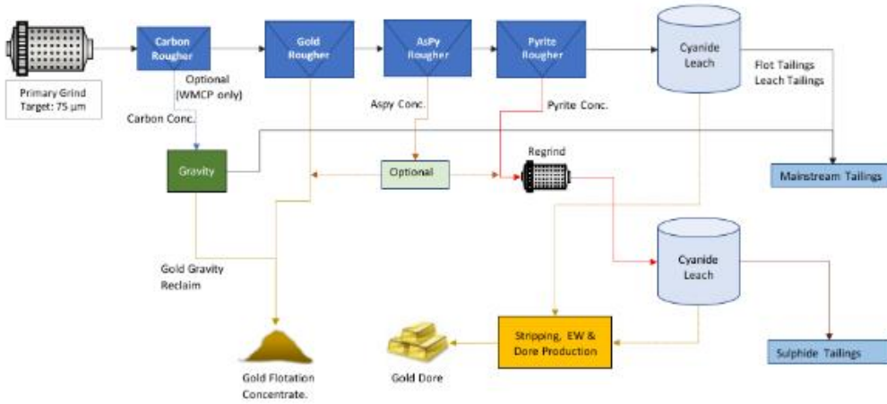
Figure STYLEREF 1 vs 10-. Flowsheet Originally Developed
